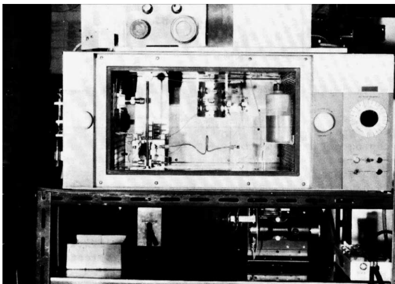
Fig. 4. The first HPLC instrument Professor Horváth built (From the collection of Csaba Horváth).
